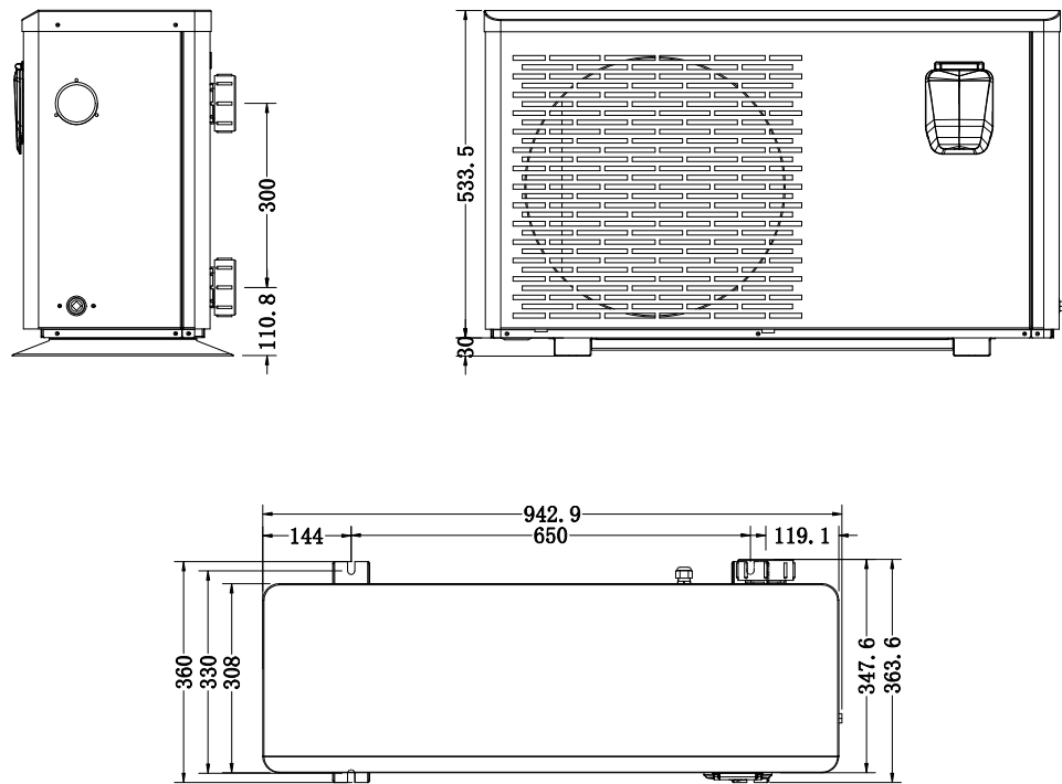
Heat pump 1402, 1403 and 1404
